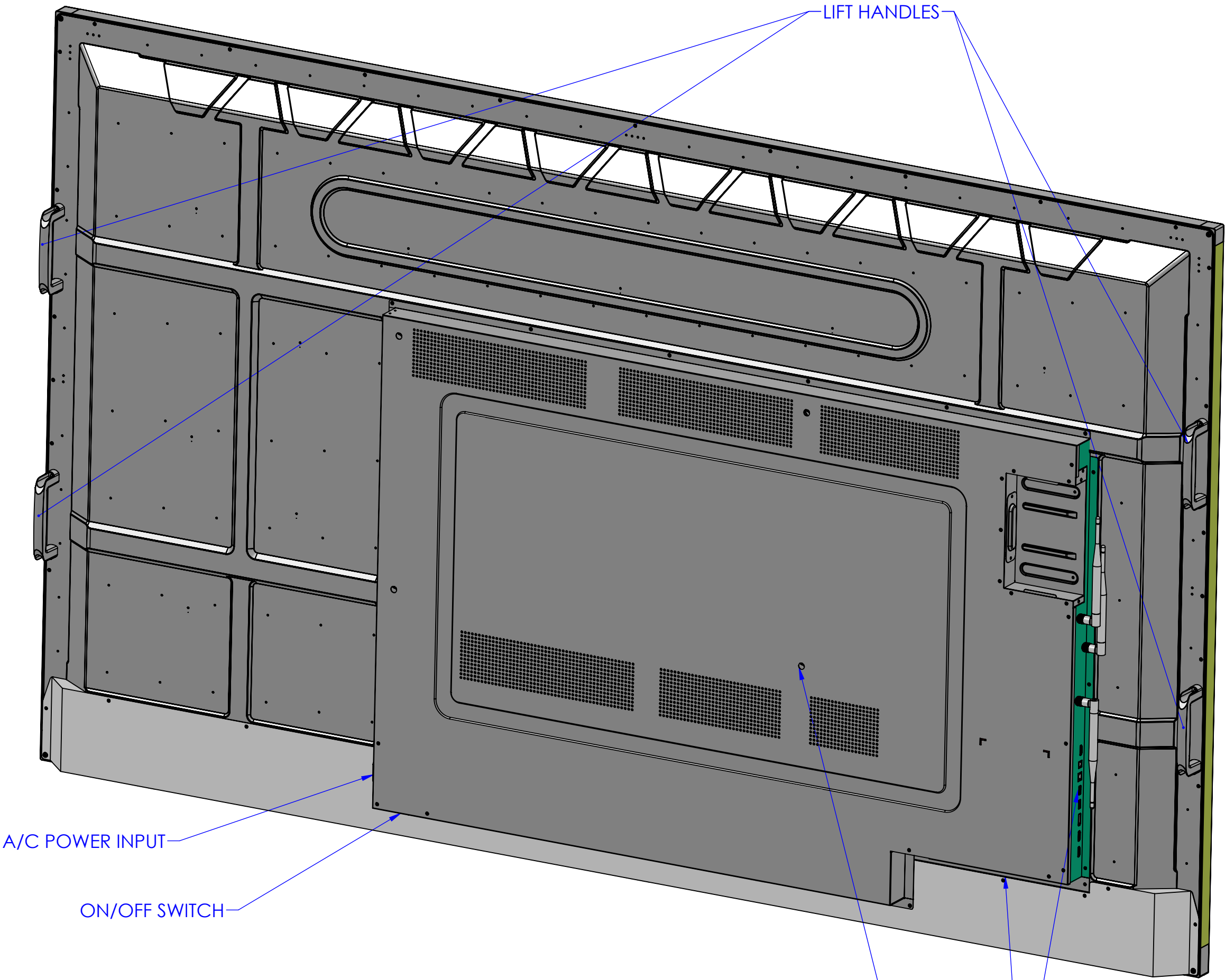
Rear Trimetric View
