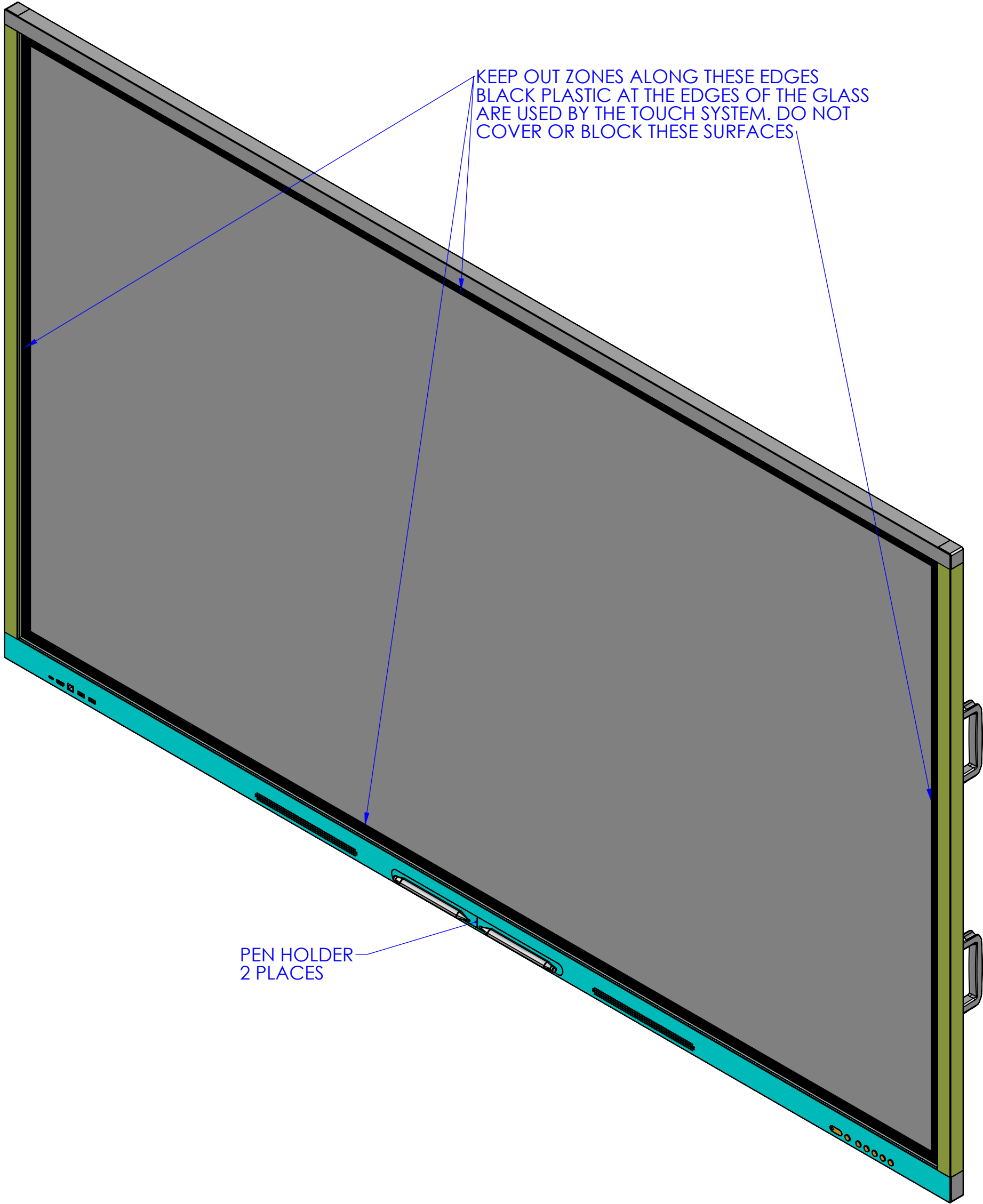
Front Trimetric View
